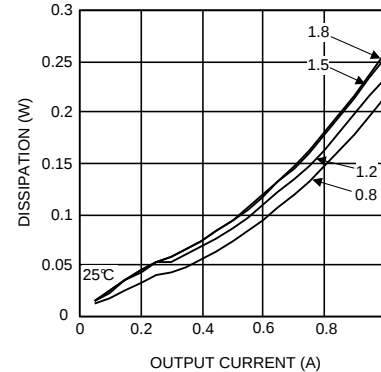
Figure 2. Dissipation 4.5-V Input at 25°C
