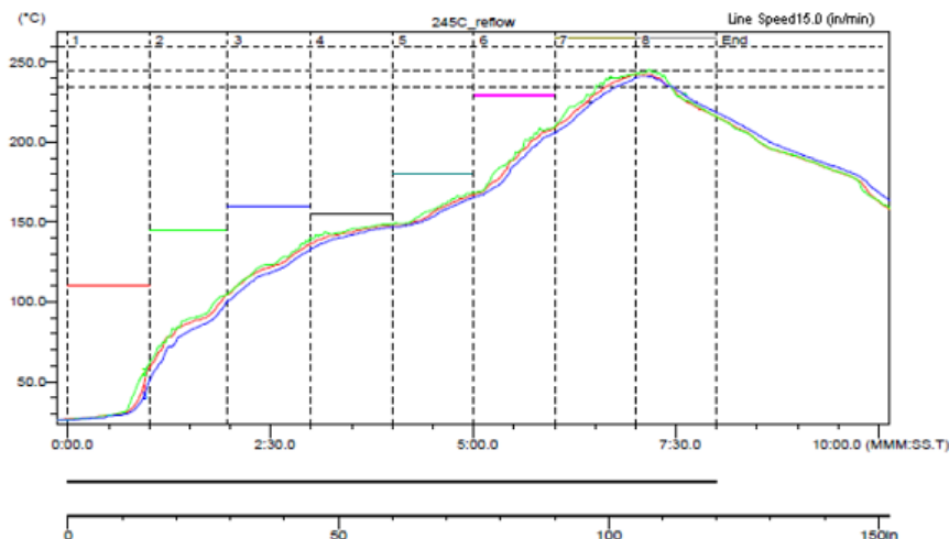
Figure 44. Sample Reflow Profile
