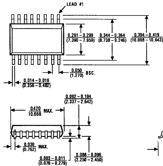
16 Lead Small Outline, Wide (WE)
