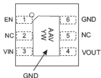
Top View DFN1.6X1.6-6L
