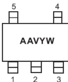
Top View SOT23-5
