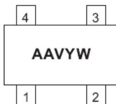
Top View SC70-4L
