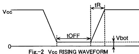
Fig.-2 Vcc RISING WAVEFORM
