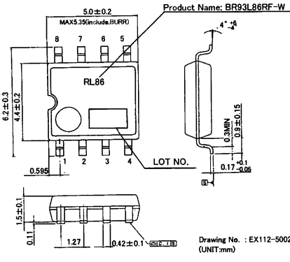
Fig4-(b) PHYSICAL DIMENSION SOP8 (BR93L86RF-W)
