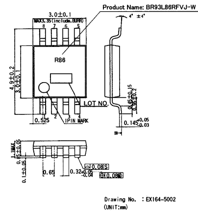
Fig4-(h) PHYSICAL DIMENSION TSSOP-B8J (BR93L86RFVJ-W)
