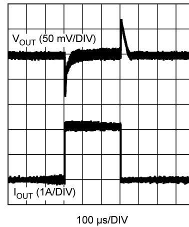
Figure 60. Transient Response I_{OUT} = 100\text{ mA} - 2A @ slewrate = 2A / \mu s
