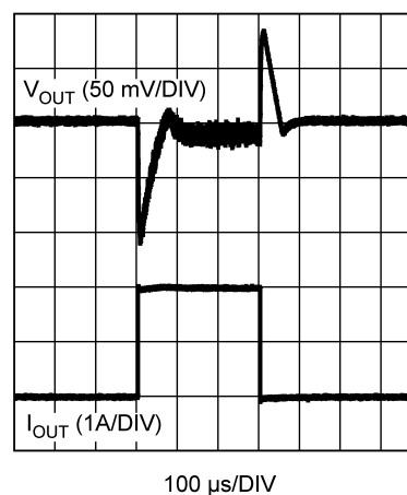
Figure 51. Transient Response I_{OUT} = 100\text{ mA} - 2A @ slewrate = 2A / \mu s
