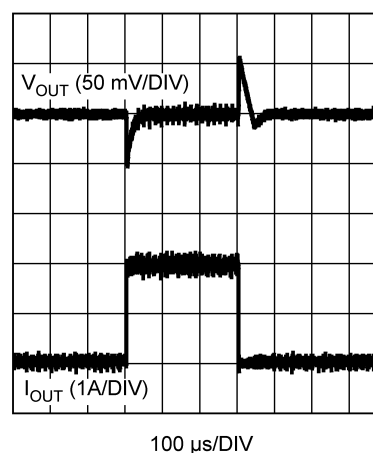
Figure 63. Transient Response I_{OUT} = 100\text{ mA} - 2A @ slewrate = 2A / \mu s
