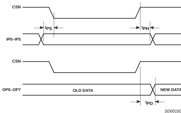
Figure 7. Port Timing
