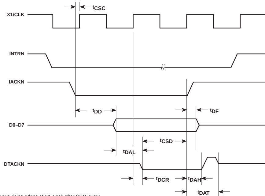
Figure 6. Interrupt Cycle Timing
