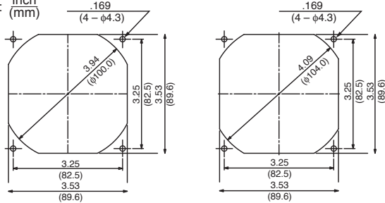
INLET SIDE
