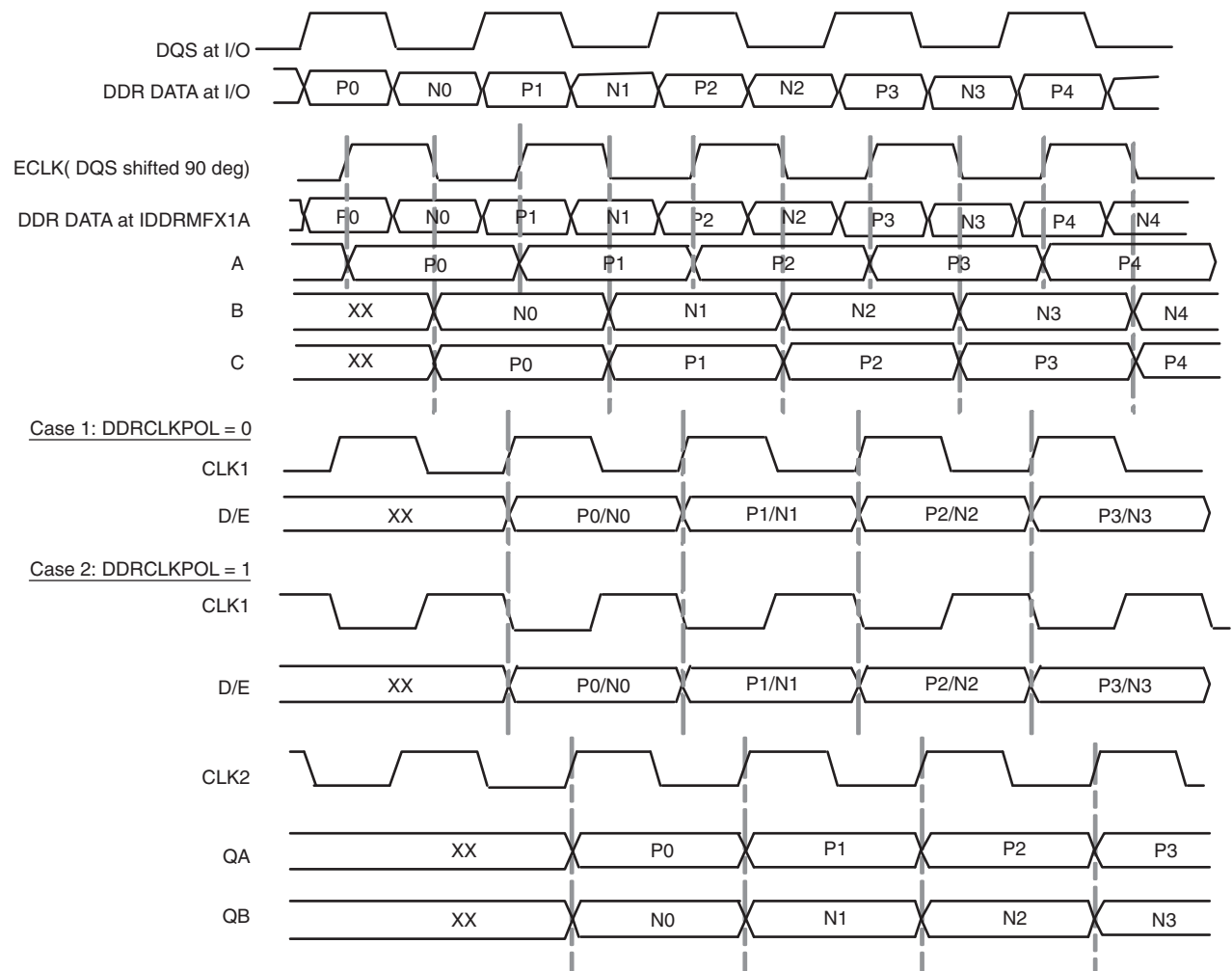
Figure 12-15. IDDRMFX1A Waveform
