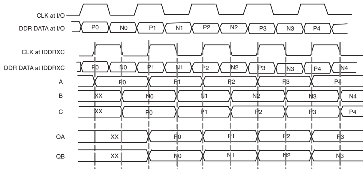
Figure 12-28. IDDRXC Waveform
