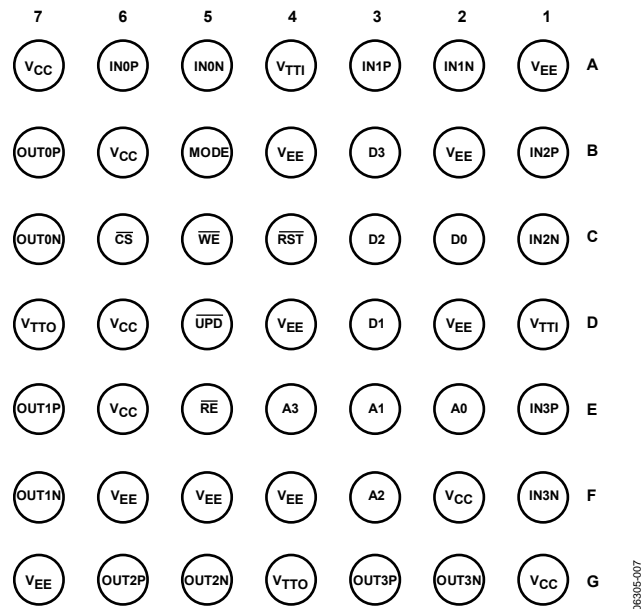
Figure 7. Pin Configuration (Bottom View)
