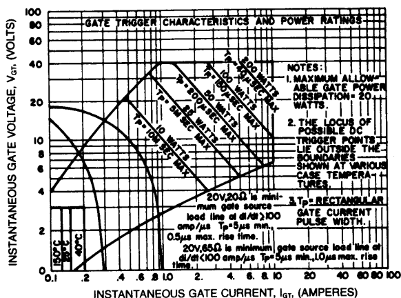
GATE CHARACTERISTICS
