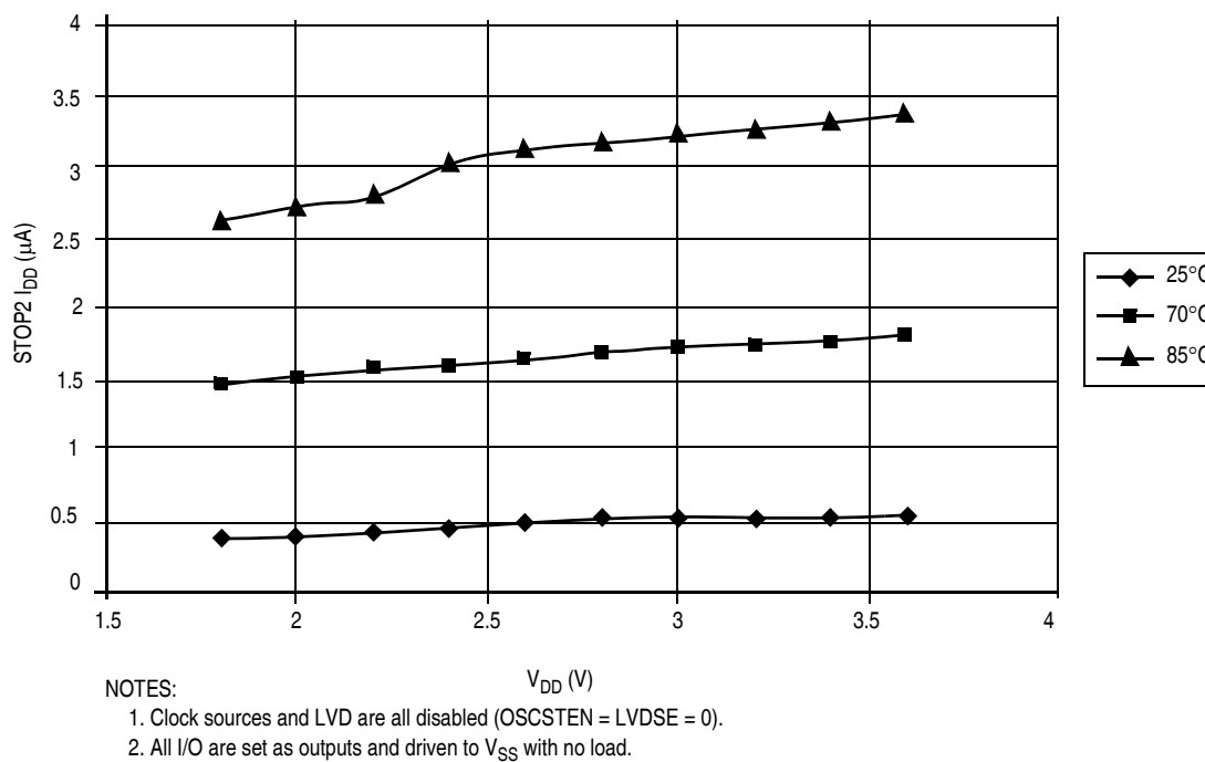
Figure A-8. Typical Stop 2 I_{DD}
