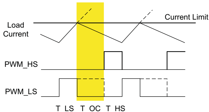
Figure 7. Cycle-by-Cycle Operation with Low Side OC (dashed line: normal operation; solid line: CBC event)
