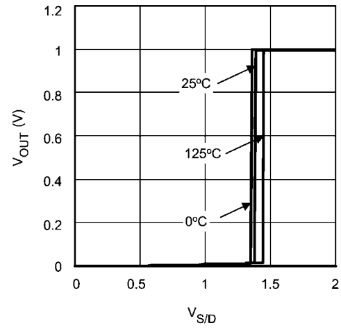
Turn-Off Characteristics
