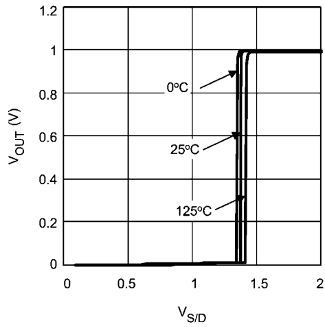
Turn-On Characteristics
