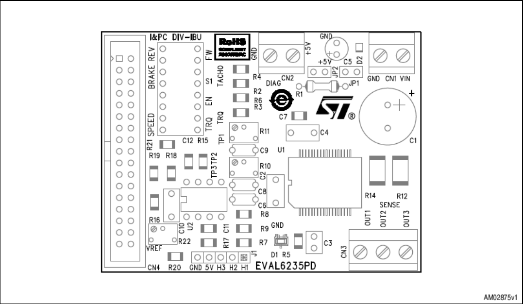
Figure 3. EVAL6235PD component placement
