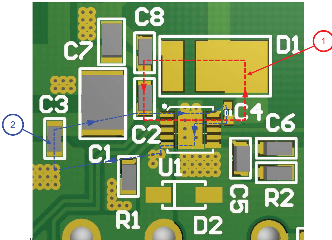
Figure 15: Example PCB Layout for Buck-Boost LED Driver Application
