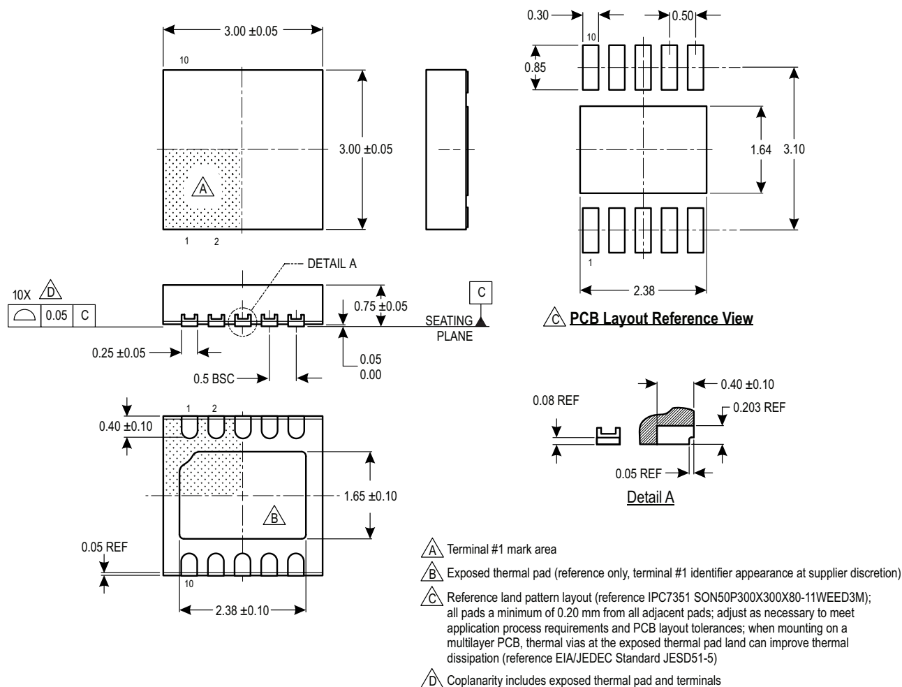
Figure 20: Package EJ, 10-Pin DFN with Exposed Thermal Pad and Wettable Flank
