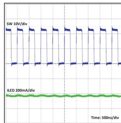
Switching Waveform
