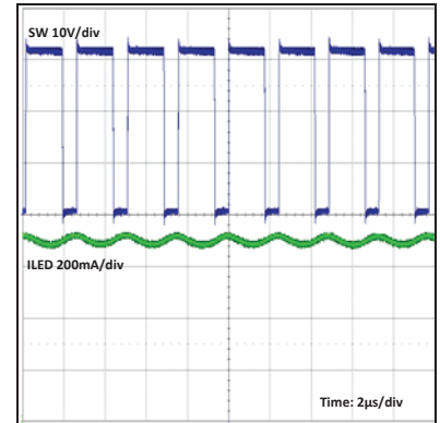
Switching Waveform
