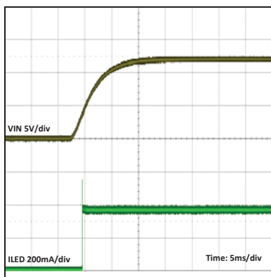
Startup Waveform
