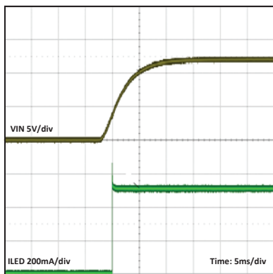
Startup Waveform
