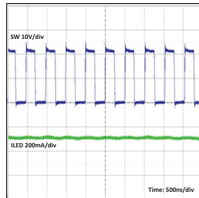
Switching Waveform
