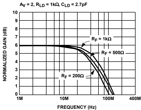
FIGURE 7. FREQUENCY RESPONSE
