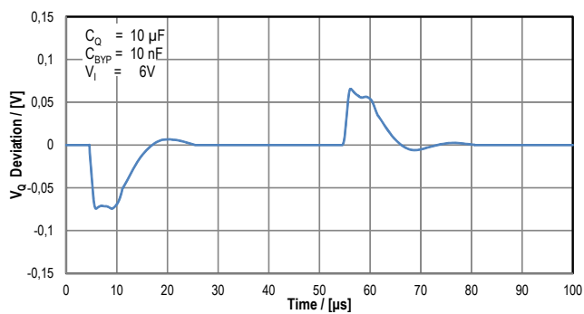
Transient Response C_{BYP} = 10 \text{ nF} (TLS205B0EJV33)
