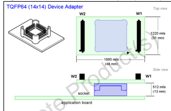
Figure 2. TQFP64 device adapter (DB543)
