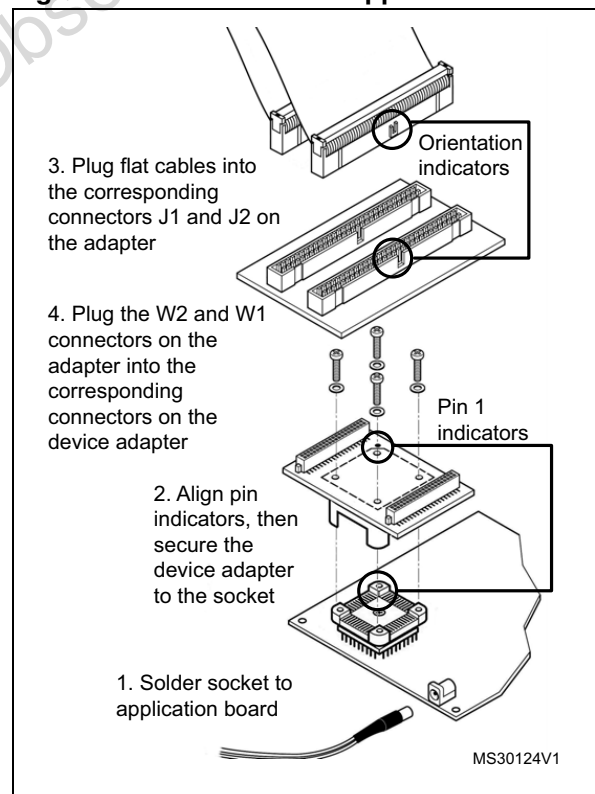
Figure 3. Connection to application board
