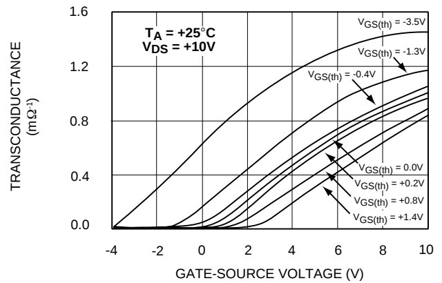
TRANSFER CHARACTERISTICS
