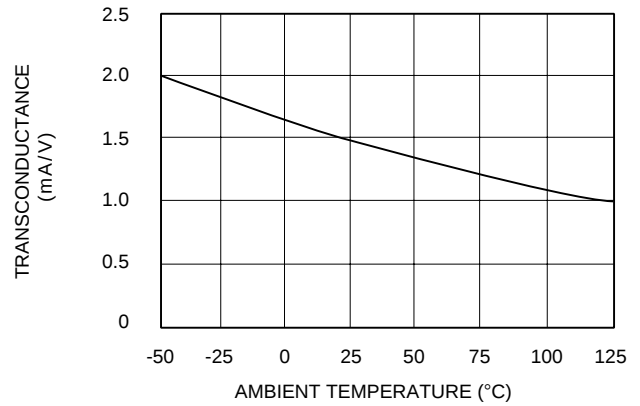
TRANSCONDUCTANCE vs. AMBIENT TEMPERATURE
