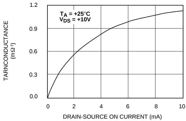
TRANCONDUCTANCE vs. DRAIN-SOURCE ON CURRENT
