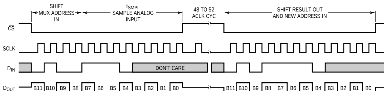
Figure 3. \overline{\text{CS}} High During Conversion
