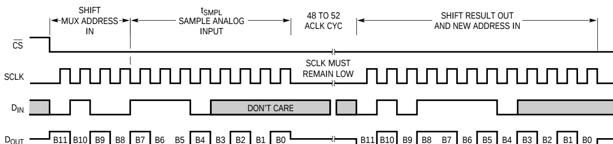
Figure 4. \overline{\text{CS}} Low During Conversion ( \overline{\text{CS}} Must go High to Low Once to Insure Proper Operation in this Mode)
