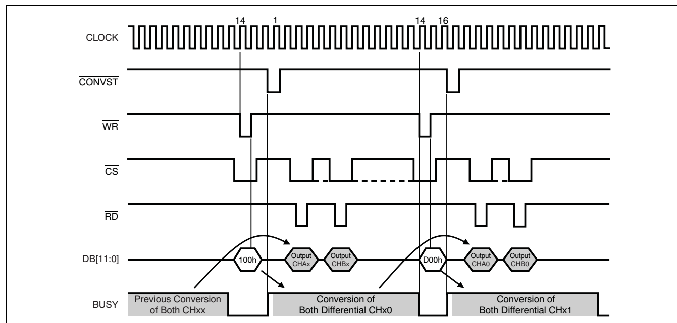
Figure 33. Channel Selection Timing Diagram
