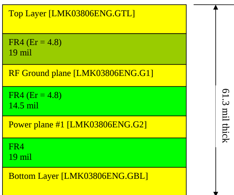
Figure 21: PCB Stackup
