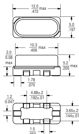
49SAB/SUB package
