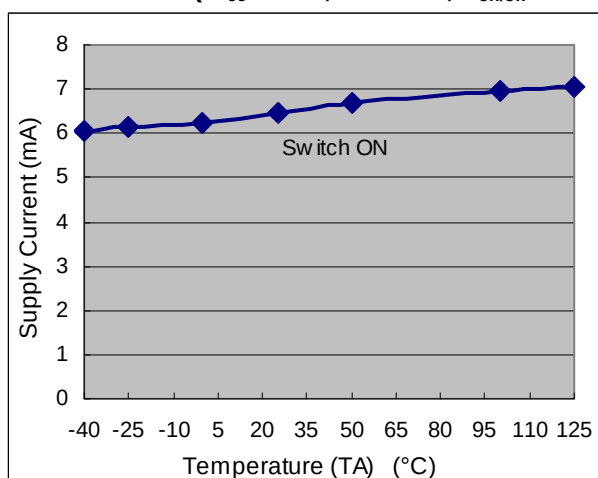
AP1512 Supply Current vs. Temperature ( V_{CC} = 12V , No Load, V_{on/off} = 0V (Switch ON), V_{on/off} = 5V (Switch OFF) )
