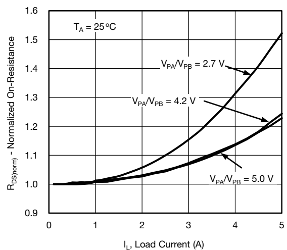
Fig. 9 - Normalized On Resistance vs. Load Current
