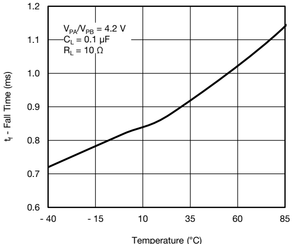
Fig. 16 - Fall Time vs. Temperature
