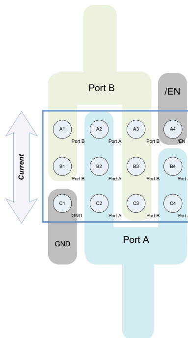
Fig. 19 - Proposed Layout
