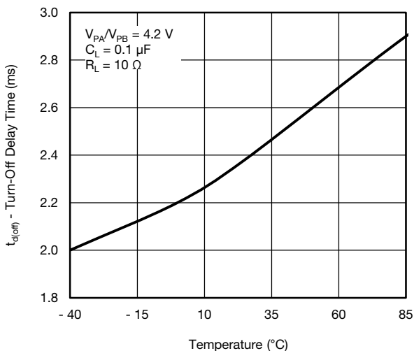
Fig. 15 - Turn-off Delay Time vs. Temperature
