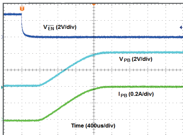
Fig. 17 - Port B Turn-On Time
