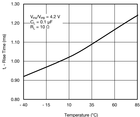
Fig. 14 - Rise Time vs. Temperature
