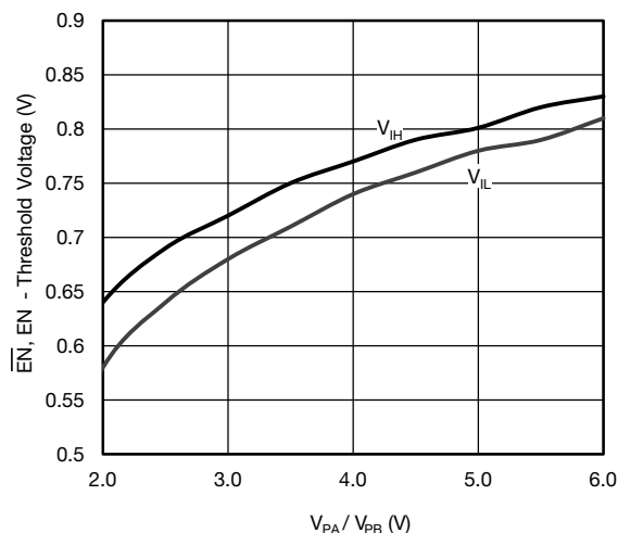
Fig. 12 - \overline{EN} , EN Threshold Voltage vs. Input Voltage
