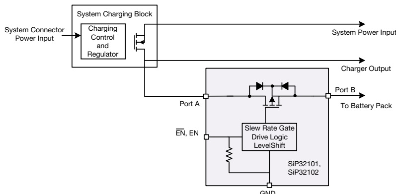
Fig. 1 - Typical Application Circuit
