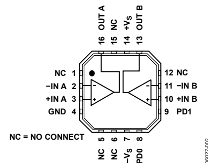
Figure 2. Thermally Enhanced, 4 mm \times 4 mm 16-Lead LFCSP_VQ
