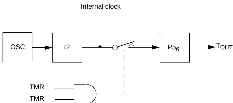
Figure 27. Internal Clock Output Using T_{OUT}
