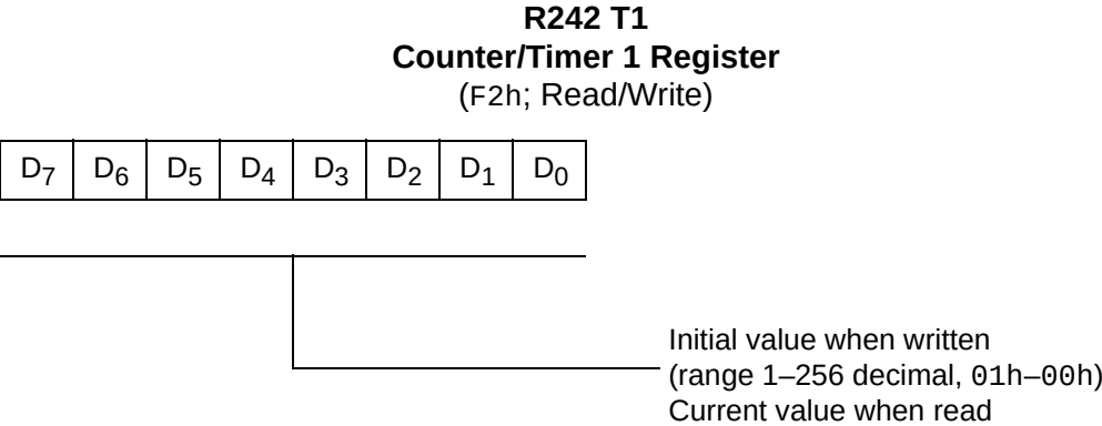
Figure 21. Counter/Timer 1 Register
