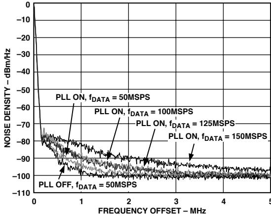
Figure 8. Phase Noise of PLL Clock Multiplier at f_{\text{OUT}} = f_{\text{DATA}}/4 at Different f_{\text{DATA}} Settings with DIV0/DIV1 Optimized, Using R&S FSEA30 Spectrum Analyzer, RBW = 30 kHz
