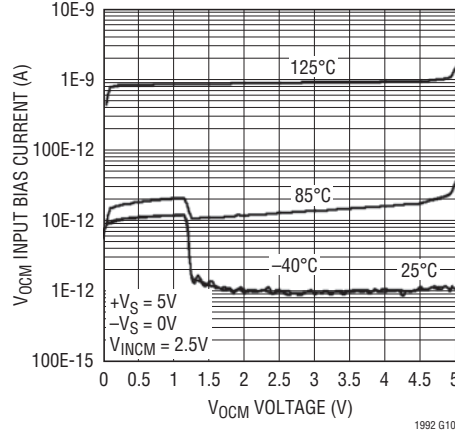
V_{OCM} Input Bias Current vs V_{OCM} Voltage
