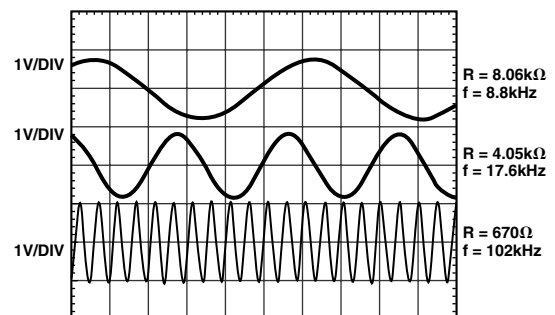
Figure 22. Programmable Oscillation
