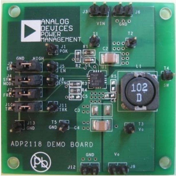
Figure 21. Evaluation Board
