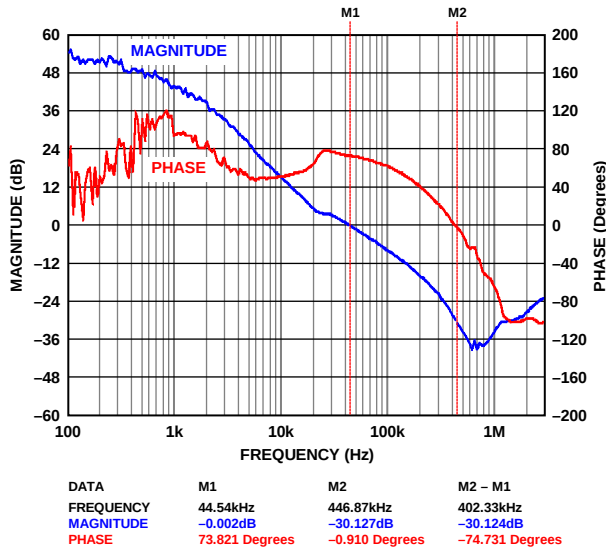
Figure 5. Bode Plot Without C_{FF}
