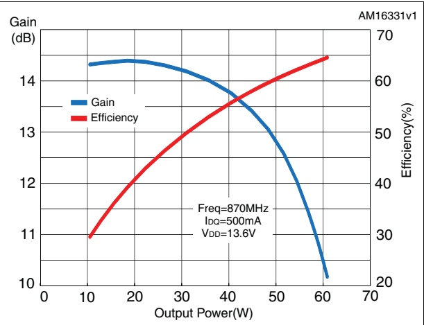
Figure 6. Gain and efficiency vs P_{OUT} - high efficiency 50 W loadline @ 13.6 V
