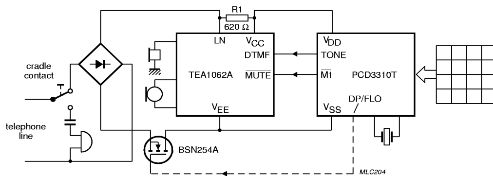
(a) DTMF pulse set with CMOS bilingual dialling circuit PCD3310T. The dashed line shows an optional flash (register recall by timed loop break).
