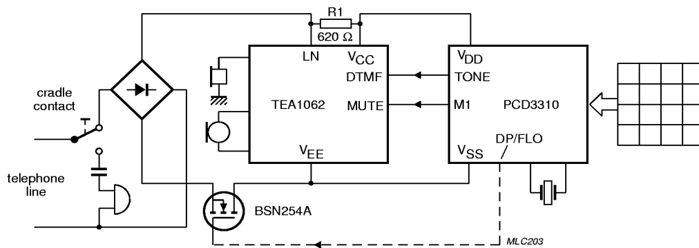
(a) DTMF pulse set with CMOS bilingual dialling circuit PCD3310. The dashed line shows an optional flash (register recall by timed loop break).
