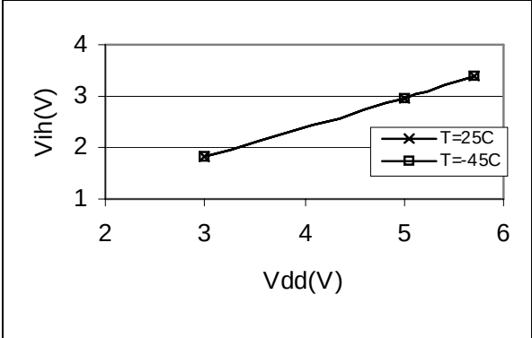
Figure 85. Typical V_{IH}
