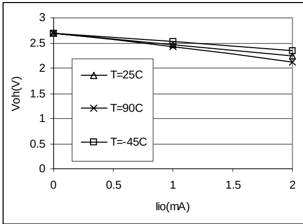
Figure 93. Typ. V_{OH} at V_{DD}=4V
