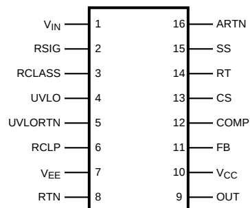
Figure 2. 16 Lead TSSOP/WSOP See Package Number PW or NHQ0016A
