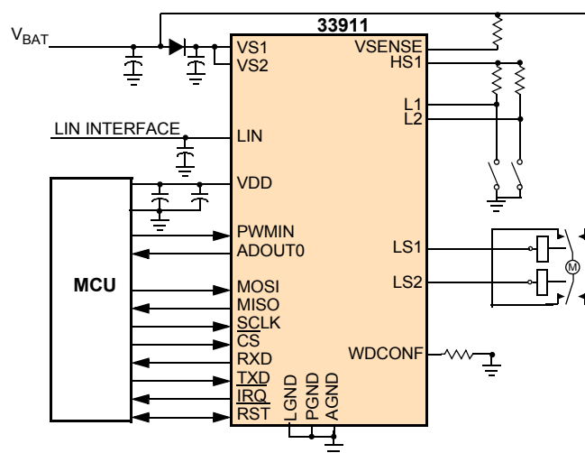
Figure 1. 33911 Simplified Application Diagram
