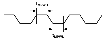
Figure 3. MCLK_I Timing
