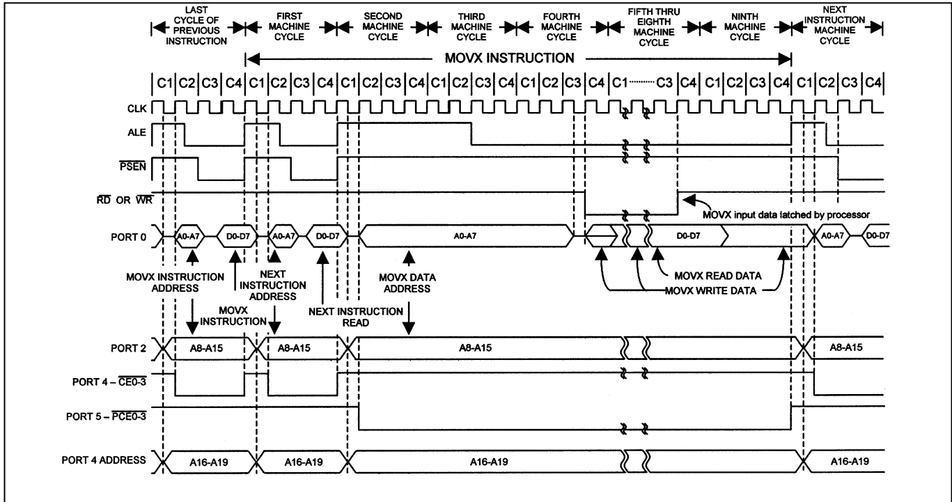
Figure 10. Multiplexed 9-Cycle Data Memory \overline{\text{PEC0-3}} Read or Write
