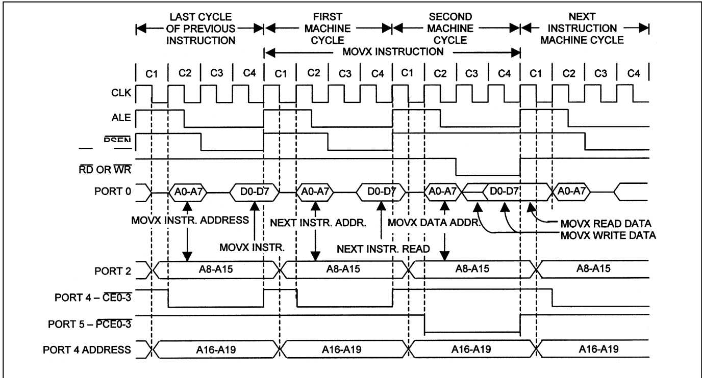
Figure 4. Multiplexed 2-Cycle Data Memory \overline{\text{PCE0-3}} Read or Write
