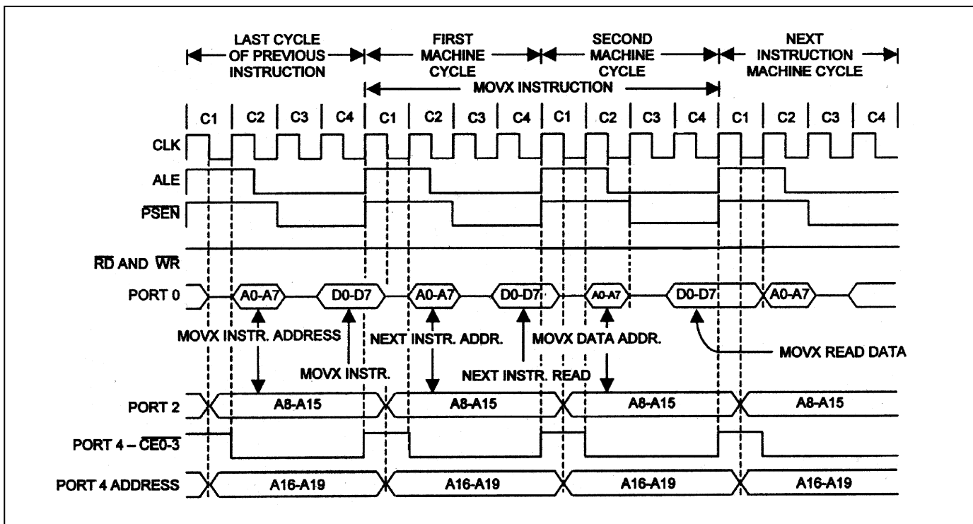
Figure 5. Multiplexed 2-Cycle Data Memory \overline{\text{CE0-3}} Read
