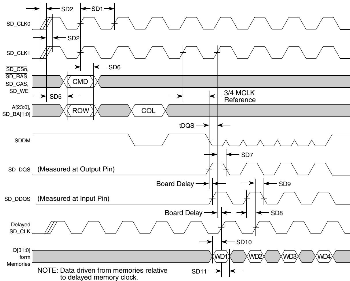
Figure 17. SDR Read Timing
