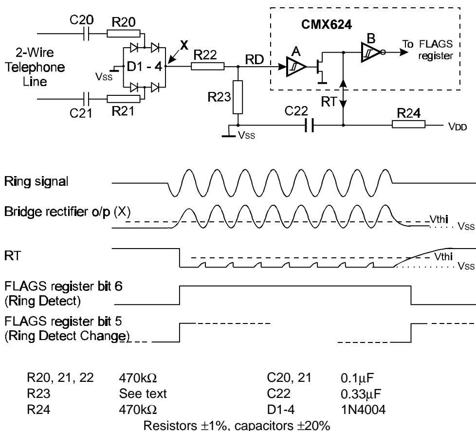
Figure 9 Ring Signal Detector Interface Circuit
