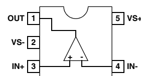
EL5192 (5 LD SOT-23) TOP VIEW
