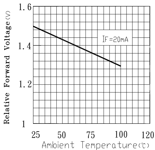
Fig. 8 Forward Voltage vs. Ambient Temperature
