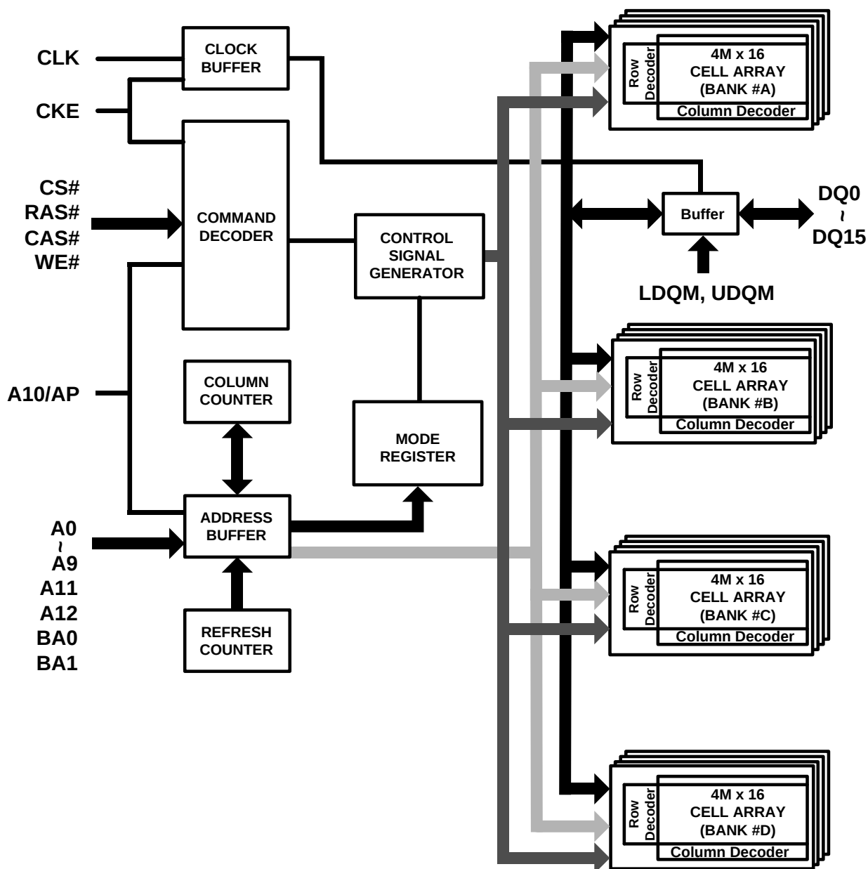
Figure 2. Block Diagram
