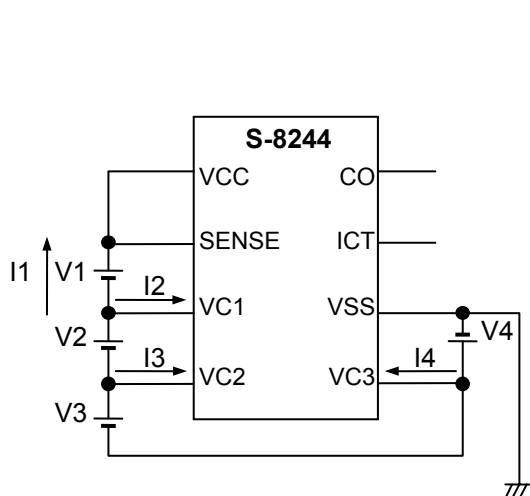
Test Circuit 3
