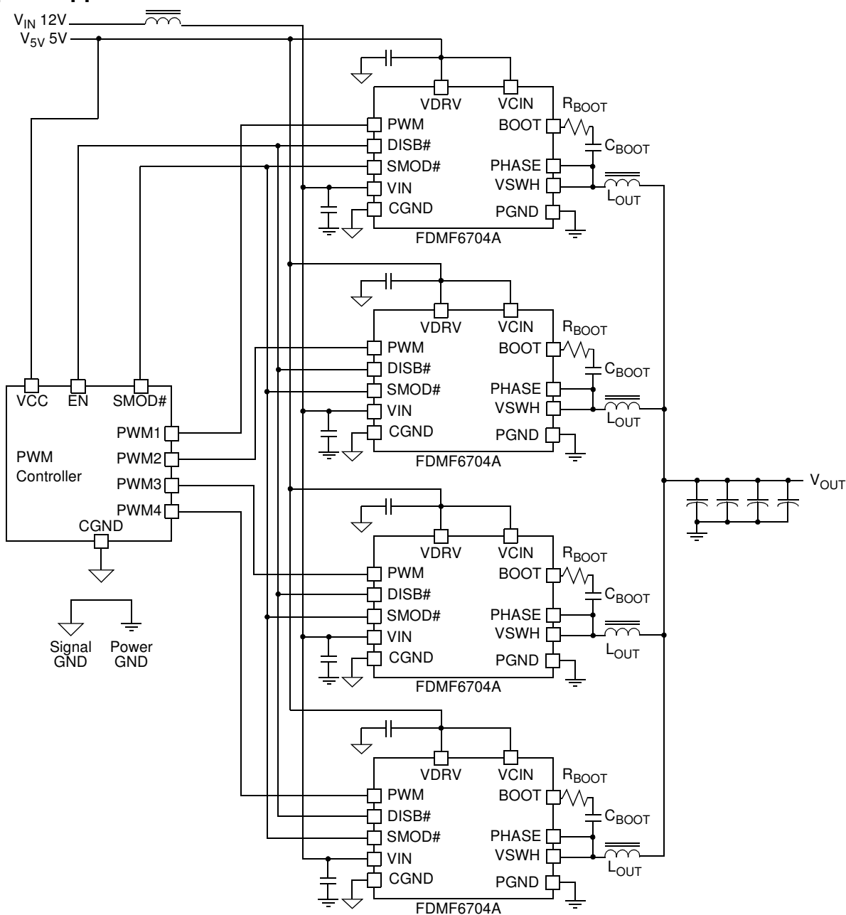
Figure 23. Typical Application
