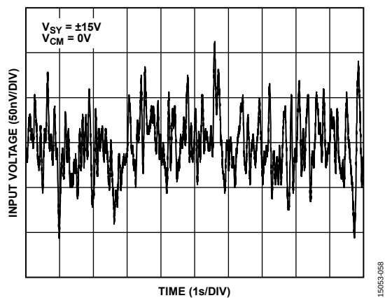
Figure 52. 0.1 Hz to 10 Hz Noise, V_{SY} = \pm 15V
