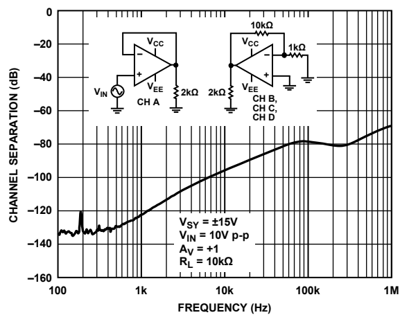
Figure 56. Channel Separation, V_{SY} = \pm 15V
