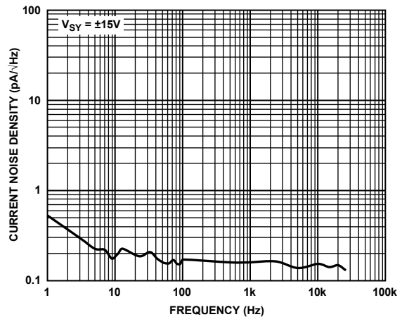
Figure 57. Current Noise Density vs. Frequency, V_{SY} = \pm 15V
