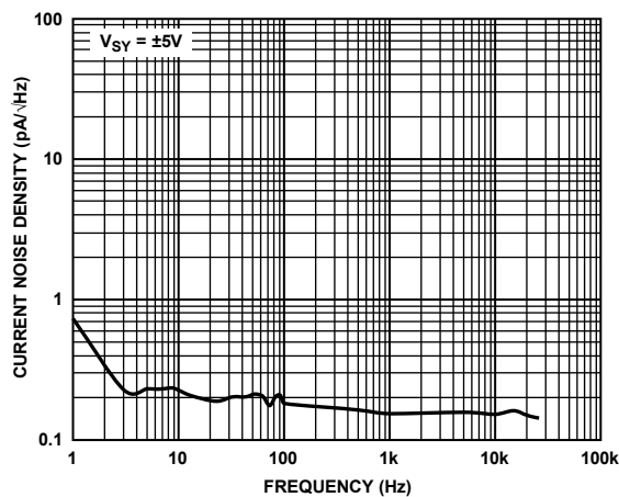
Figure 54. Current Noise Density vs. Frequency, V_{SY} = \pm 5V
