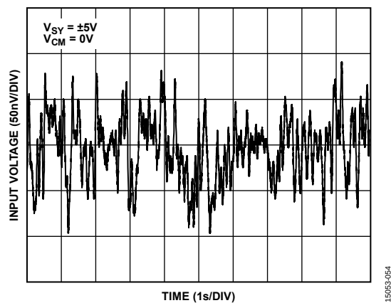
Figure 55. 0.1 Hz to 10 Hz Noise, V_{SY} = \pm 5V
