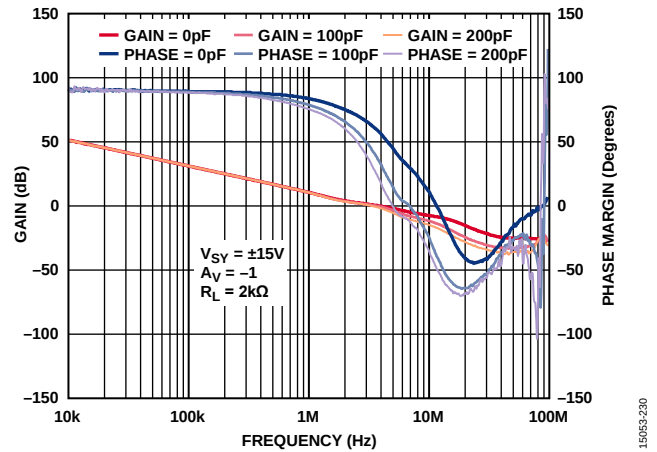
Figure 25. Open-Loop Gain and Phase Margin vs. Frequency, V_{SY} = \pm 15 V
