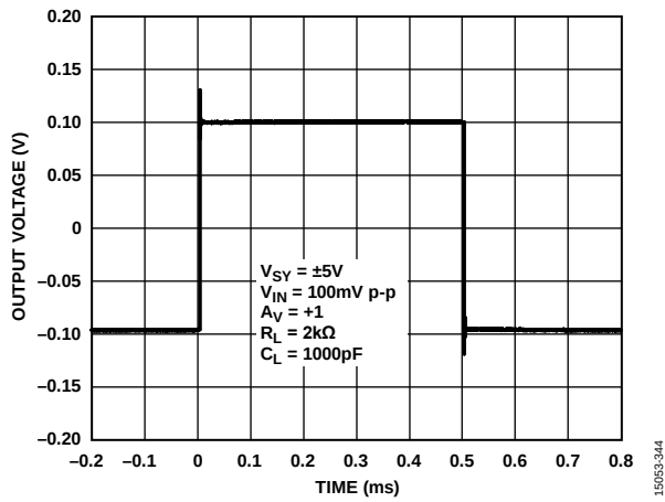
Figure 35. Small Signal Transient Response, V_{SY} = \pm 5V
