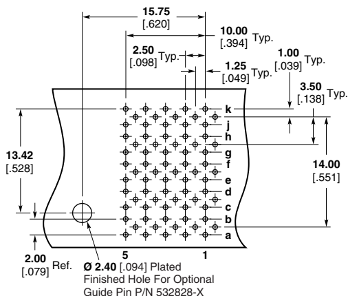
Recommended PC Board Layout (Component Side Shown) For Non-Midplane Applications For Midplane Applications Reference Page 74
