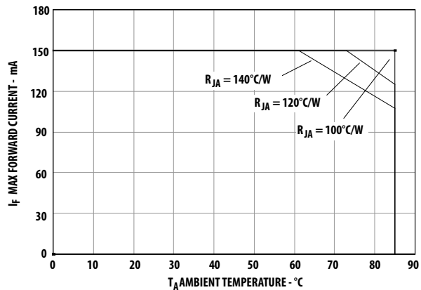
Figure 5. Maximum forward current vs. ambient temperature. Derated based on T_{J\text{MAX}} = 145^{\circ}\text{C} , R_{\theta JA} = 100^{\circ}\text{C/W} , 120^{\circ}\text{C/W} and 140^{\circ}\text{C/W}
