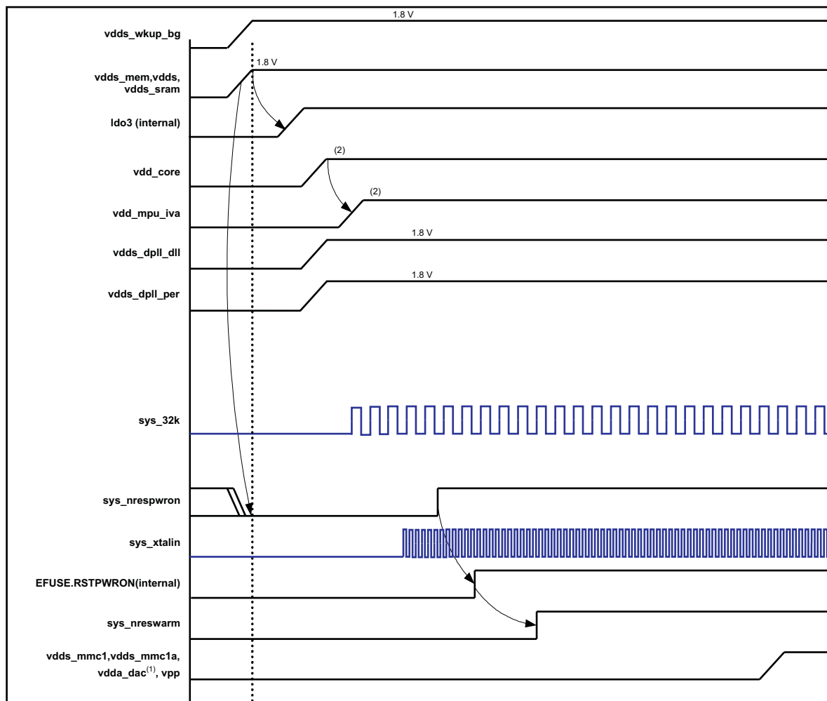
Figure 3-3. Power-up Sequence
