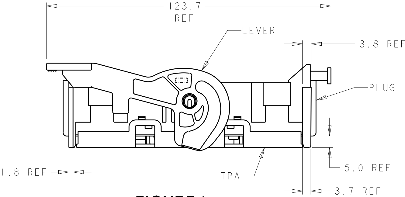
FIGURE 1 1326073-1 KEYING OPTION A
